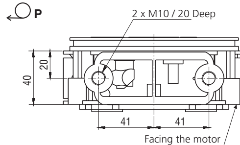
Connecting Holder
