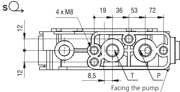
Connecting Block
