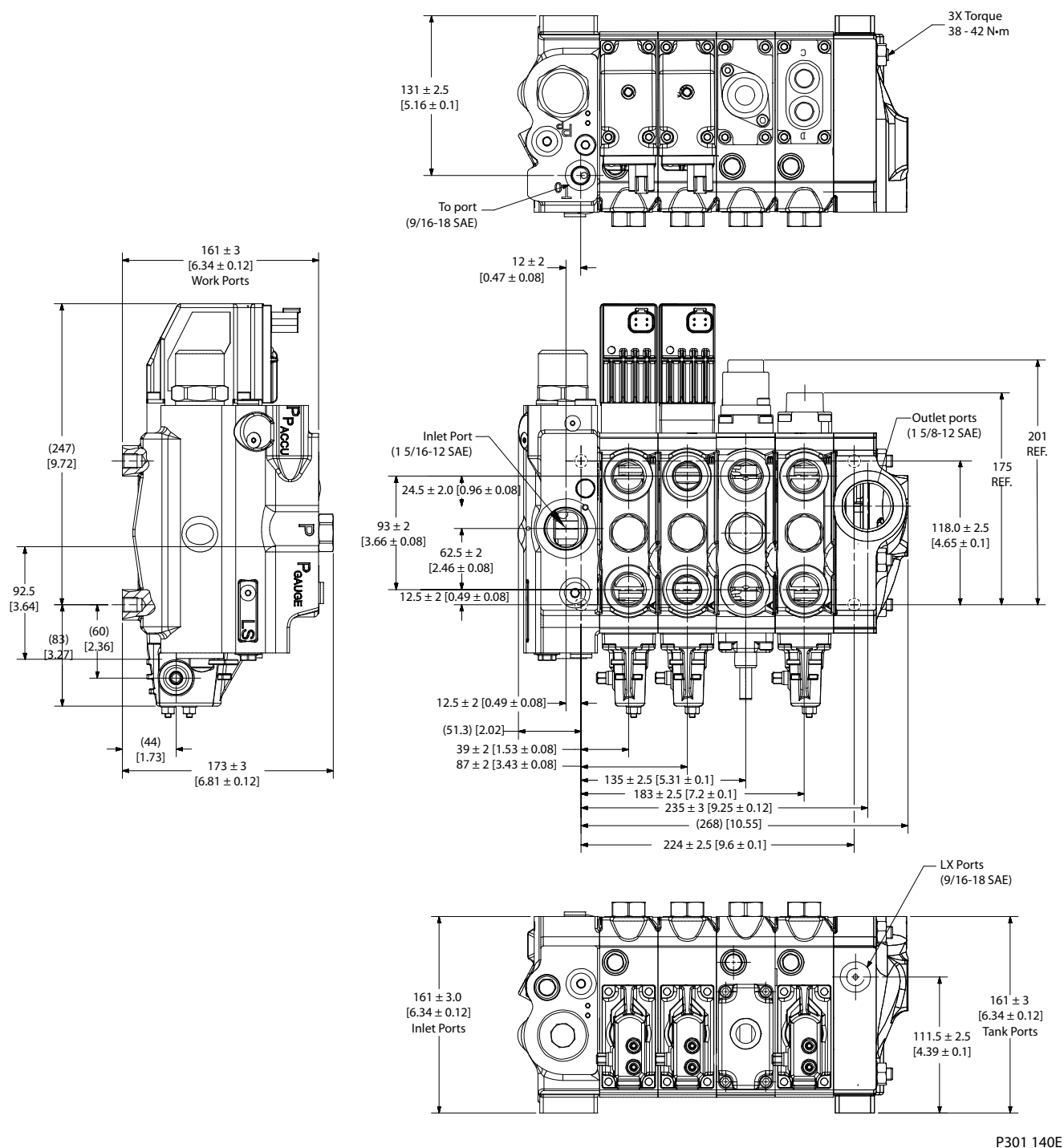
PVG 100 with variable displ. pump
