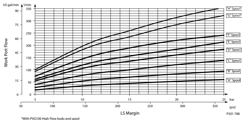
Flow vs. LS margin @ maximum spool shift
